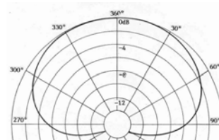
Horizontal Plane
