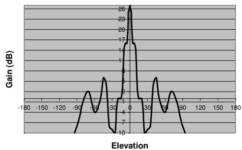
Vertical Radiation Pattern
